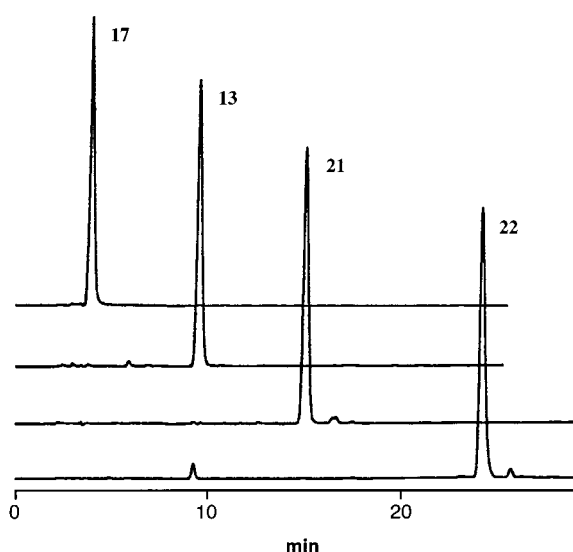
Figure 1. RP-HPLC traces of free (13 and 17) and terminally protected (21 and 22) acids (C 18 column; absorbance at 220 nm; linear gradient: cf. Experimental Section)
