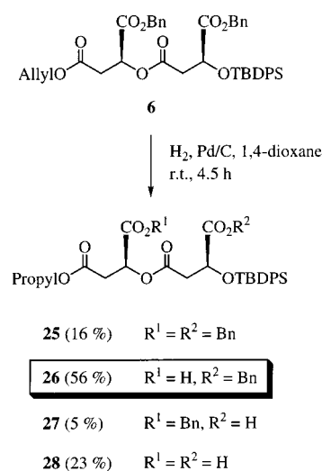
Scheme 9. Preferred cleavage of one of the benzyl ester groups in 6
