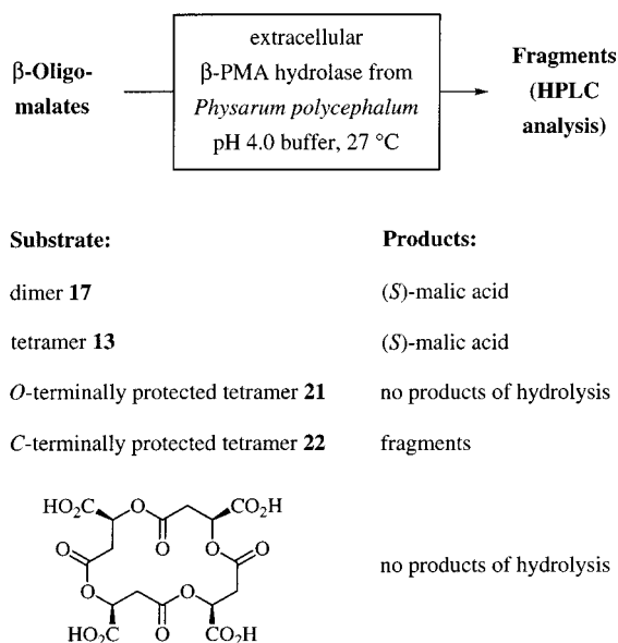
Figure 2. Enzymatic degradation of oligomers 13 , 17 , 21 , and 22 , and of a cyclic tetramer (an X-ray crystal structure of the tetra-benzyl ester [24] of this tetramer was determined; the coordinates can be provided at request to the correspondence author)
