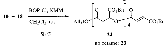
Scheme 9. Preferred cleavage of one of the benzyl ester groups in 6
