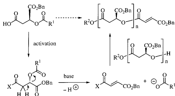
Scheme 8. \beta -Elimination prior to acylation in the case of carboxylic acid activation in the presence of a base
