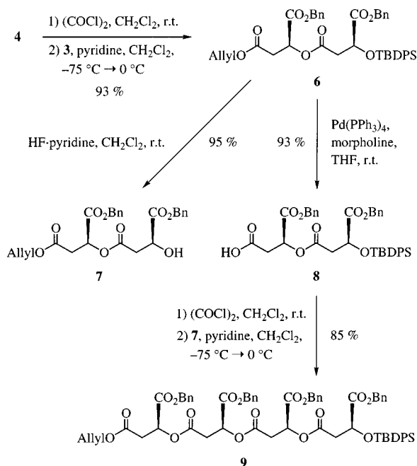
Scheme 3. Formation and selective deprotection of 6, followed by segment coupling of the dimer moieties 7 and 8
