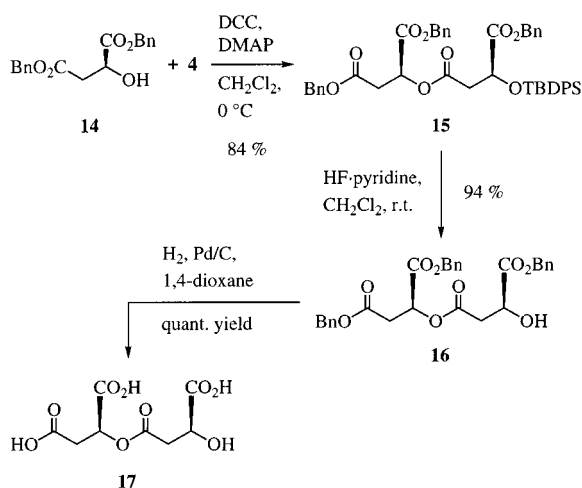
Scheme 5. Preparation of dimer 17
