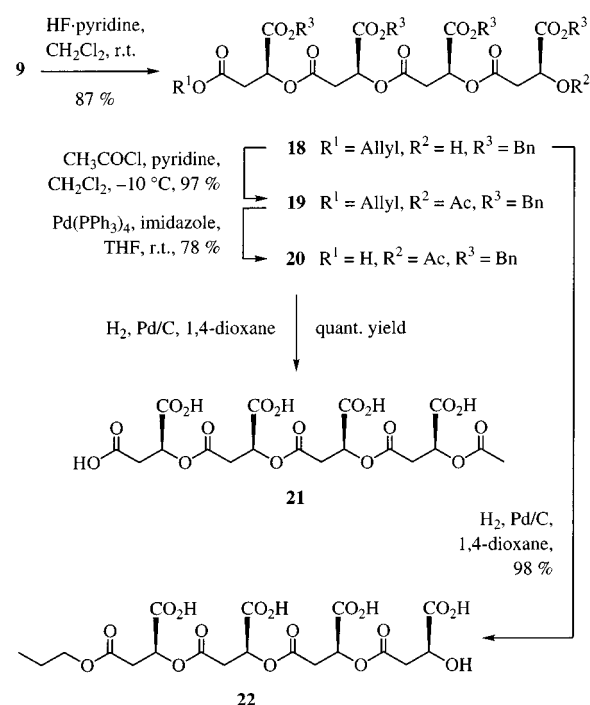
Scheme 6. Synthesis of terminally protected tetramers 21 and 22
