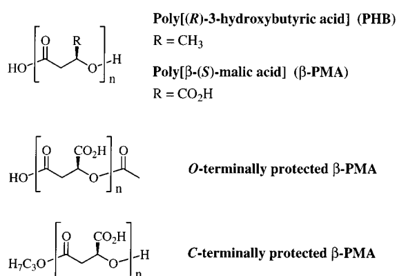
Scheme 1. Linear oligomers of 3-hydroxyalkanoic acids and of malic acid
