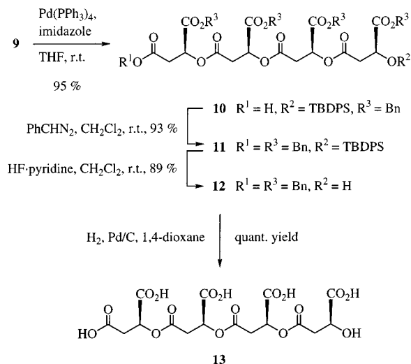
Scheme 4. Preparation of tetramer 13, involving transformation of the terminal allyl ester in 9 to a benzyl ester
