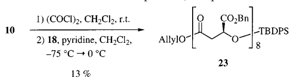
Scheme 7. Preparation of the octamer 23 by acid chloride coupling
