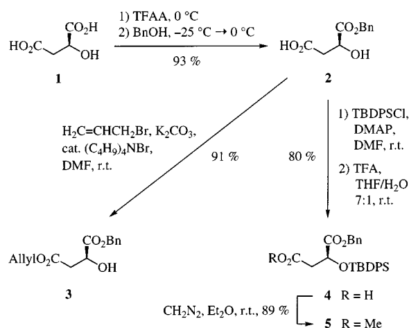
Scheme 2. Preparation of the monomers 3 and 4 by specific protection of malic acid ( 1 )
